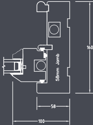
Concealed Spiral Balance
