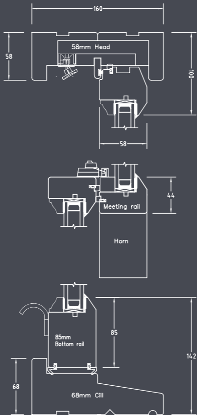
Weights & Pulleys / Concealed Spiral Balance
